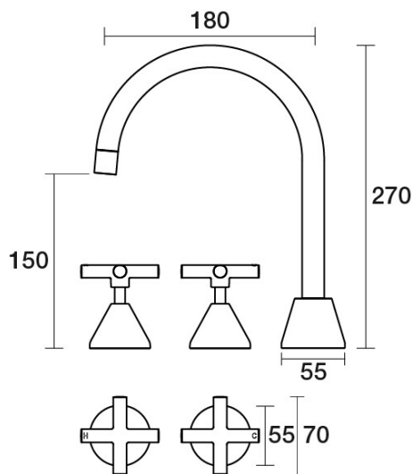
Poem Spa Set Hob Swivel B30.061.1.39 - Antique Bronze
