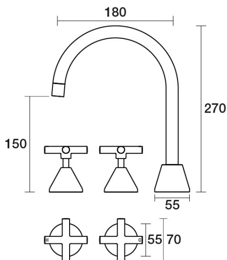
Poem Spa Set Hob Swivel Ceramic Disc B30.061.2.44 - Antique Copper
