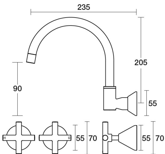
Poem Spa Set Wall Swivel B30.062.1.21 - Brushed Rose Gold
