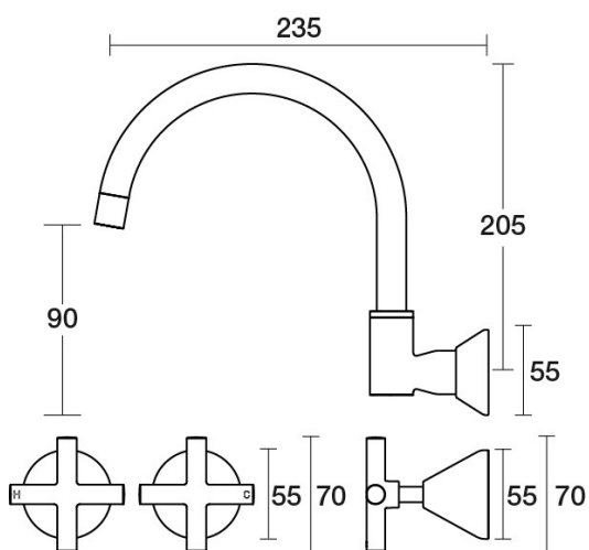
Poem Spa Set Wall Swivel B30.062.1.47 - Luminick
