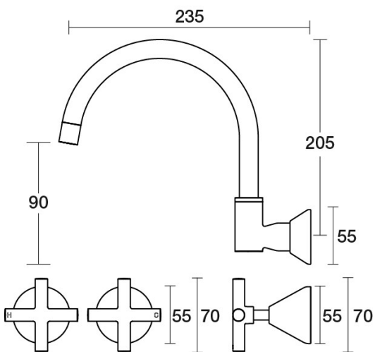
Poem Spa Set Wall Swivel Ceramic Disc B30.062.2.42 - Brushed Copper
