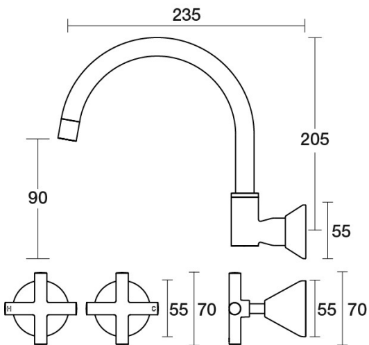
Poem Spa Set Wall Swivel Ceramic Disc B30.062.2.43 - Brass
