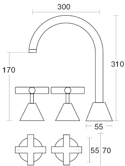
Poem Spa Set XL Hob Swivel Ceramic Disc B30.063.2.01 - Chrome
