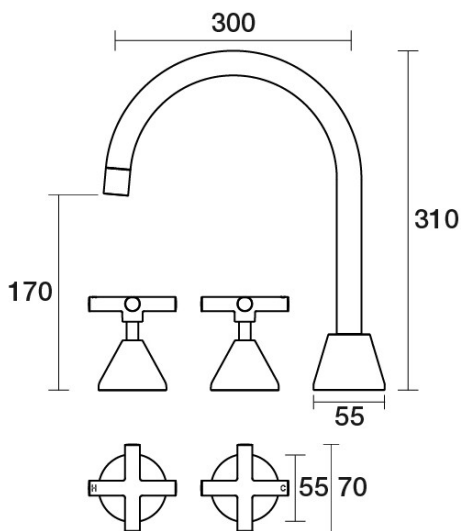
Poem Spa Set XL Hob Swivel Ceramic Disc B30.063.2.27 - Satin Pearl
