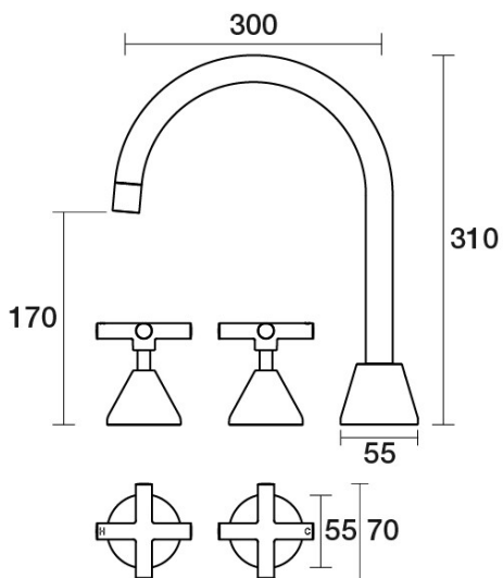
Poem Spa Set XL Hob Swivel Ceramic Disc B30.063.2.40 - Rumbled Brass
