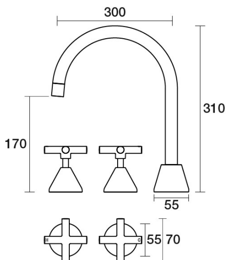
Poem Spa Set XL Hob Swivel Ceramic Disc B30.063.2.41 - Brushed Brass
