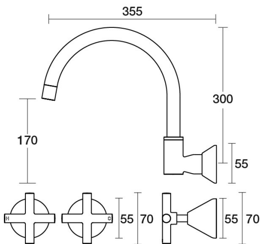
Poem Spa Set XL Wall Swivel B30.064.1.19 - 23k Brushed Brass Gold
