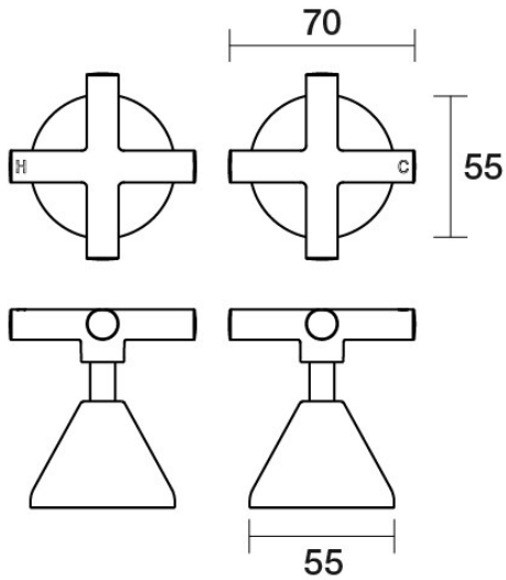
Poem Top Assemblies Wall Pair Ceramic Disc B30.082.2.01 - Chrome
