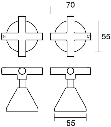
Poem Top Assemblies Wall Pair Ceramic Disc B30.082.2.42 - Brushed Copper
