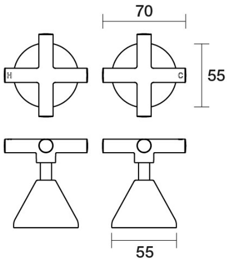
Poem Top Assemblies Wall Pair Ceramic Disc B30.082.2.52 - Burnished
