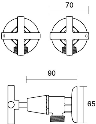
Poem Washing Machine Stops Wall Pair B30.091.1.67 - Vintage Brass
