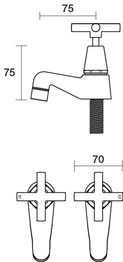
Poem Pillar Taps Pair B30.111.1.48 - Copper
