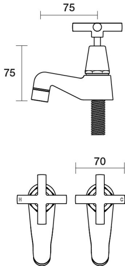
Poem Pillar Taps Pair B30.111.1.57 - Matt Nickel
