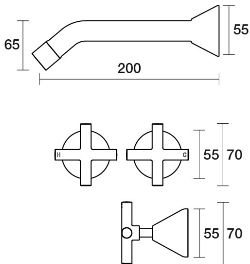
Poem Wall Basin Set 200mm Outlet B30.152.1.45 - Native Brass
