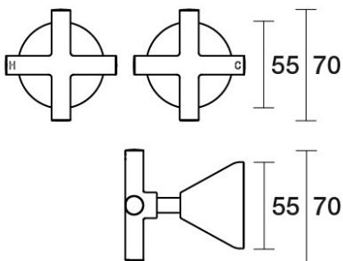
Poem Wall Basin Set 200mm Outlet Ceramic Disc B30.152.2.57 - Matt Nickel
