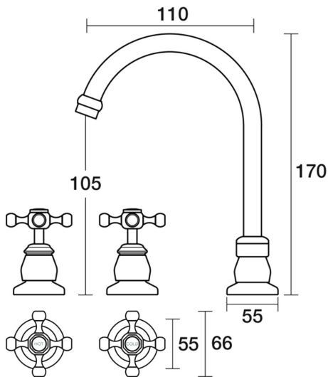
Tudor Basin Set Swivel B31.011.1.32 - Midnight Black
