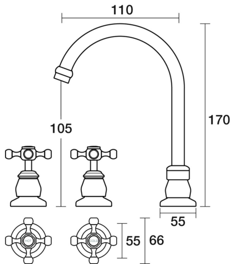
Tudor Basin Set Swivel B31.011.1.41 - Brushed Brass
