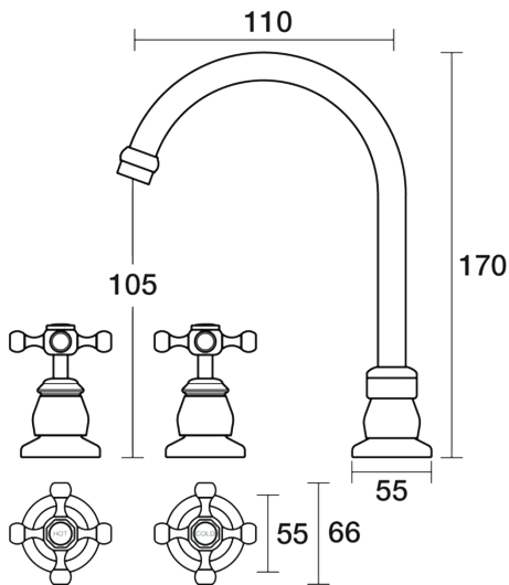
Tudor Basin Set Swivel Ceramic Disc B31.011.2.01 - Chrome
