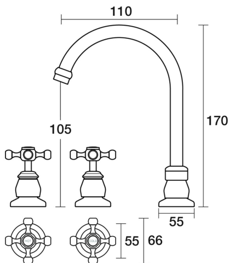
Tudor Basin Set Swivel Ceramic Disc B31.011.2.45 - Native Brass
