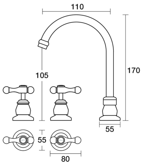
Tudor Basin Set Swivel Lever Ceramic Disc B31.011.3.02 - Brushed Chrome
