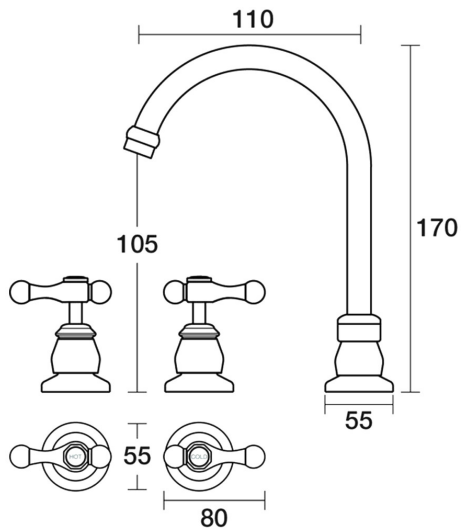
Tudor Basin Set Swivel Lever Ceramic Disc B31.011.3.40 - Rumbled Brass
