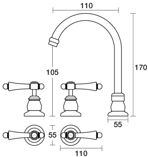
Tudor Basin Set Swivel Porcelain Lever Ceramic Disc B31.011.4.52 - Burnished
