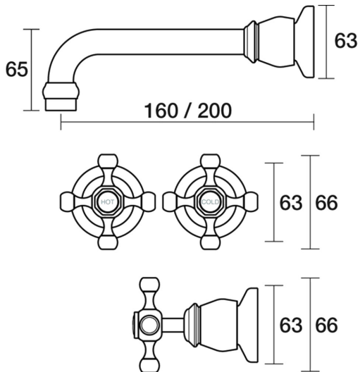
Tudor Wall Bath Set 160mm Outlet Ceramic Disc B31.021.2.57 - Matt Nickel
