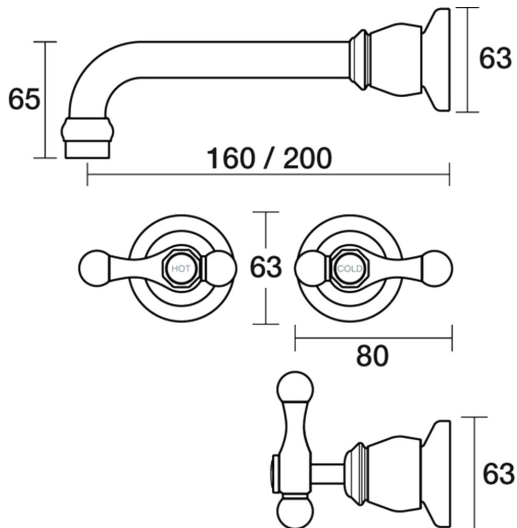
Tudor Wall Bath Set 160mm Outlet Lever Ceramic Disc B31.021.3.14 - Gold / Ivory
