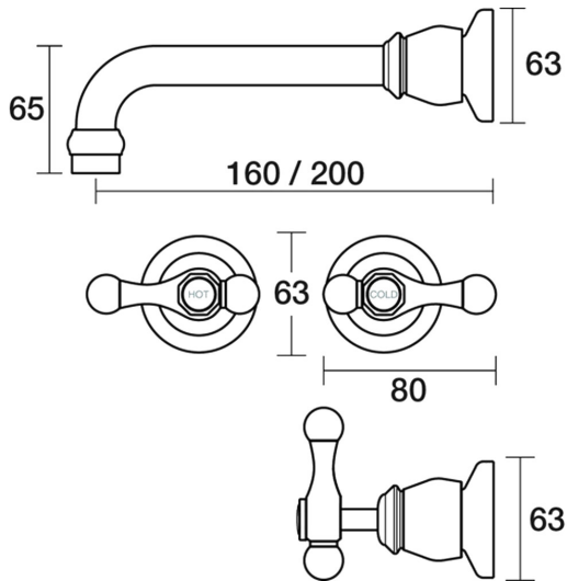
Tudor Wall Bath Set 160mm Outlet Lever Ceramic Disc B31.021.3.54 - Volcanic Grey
