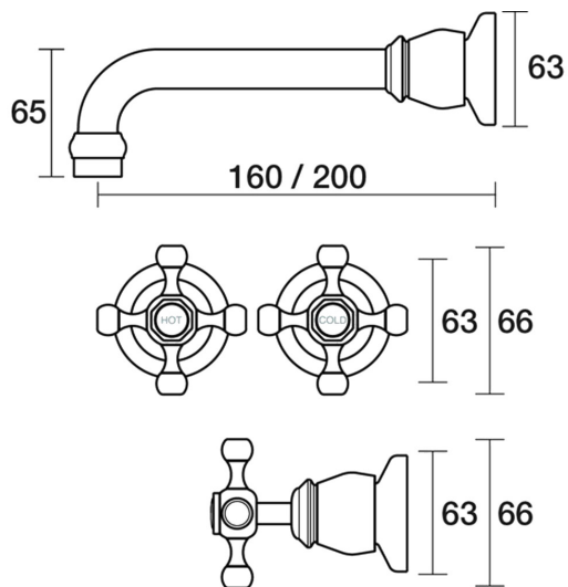
Tudor Wall Bath Set 200mm Outlet B31.022.1.03 - Chrome / White
