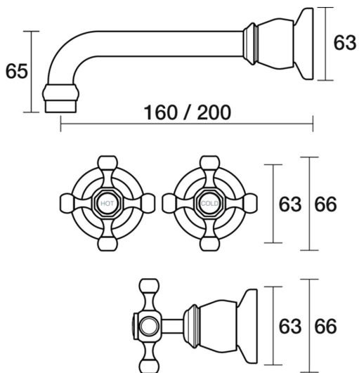
Tudor Wall Bath Set 200mm Outlet Ceramic Disc B31.022.2.25 - Brushed Nickel
