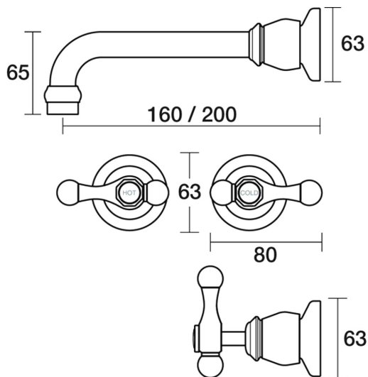
Tudor Wall Bath Set 200mm Outlet Lever Ceramic Disc B31.022.3.02 - Brushed Chrome
