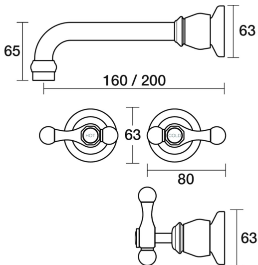
Tudor Wall Bath Set 200mm Outlet Lever Ceramic Disc B31.022.3.19 - 23k Brushed Brass Gold
