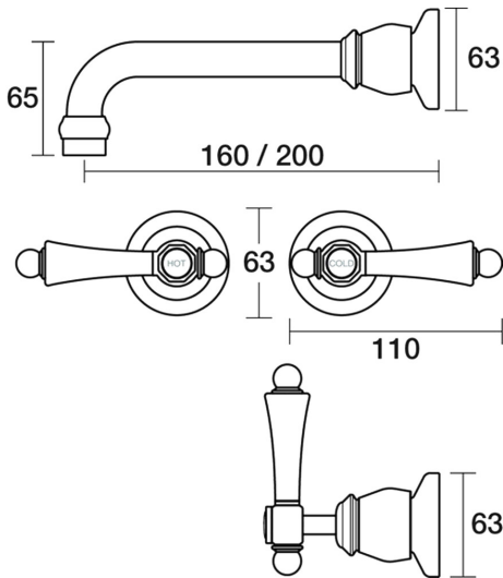
Tudor Wall Bath Set 200mm Outlet Porcelain Lever Ceramic Disc B31.022.4.11 - 23k Gold
