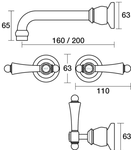
Tudor Wall Bath Set 200mm Outlet Porcelain Lever Ceramic Disc B31.022.4.23 - Gunmetal
