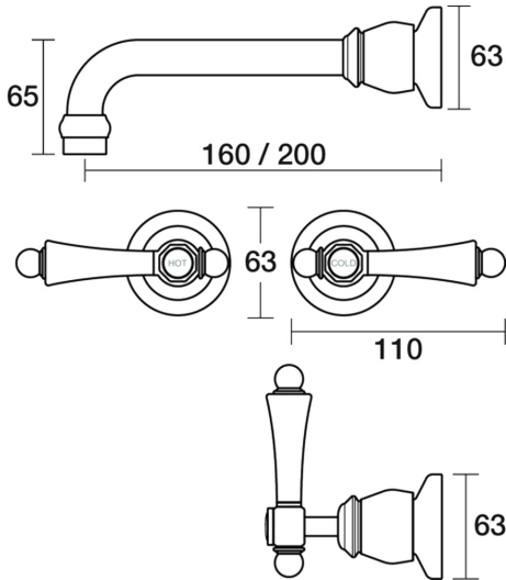
Tudor Wall Bath Set 200mm Outlet Porcelain Lever Ceramic Disc B31.022.4.43 - Brass
