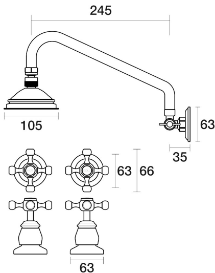
Tudor Shower Set Adjustable Arm Ceramic Disc B31.031.2.11 - 23k Gold
