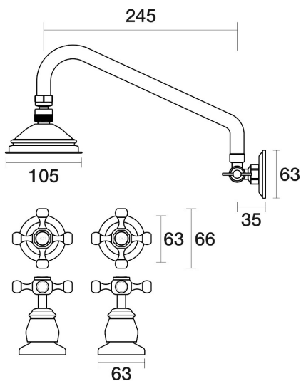
Tudor Shower Set Adjustable Arm Ceramic Disc B31.031.2.32 - Midnight Black
