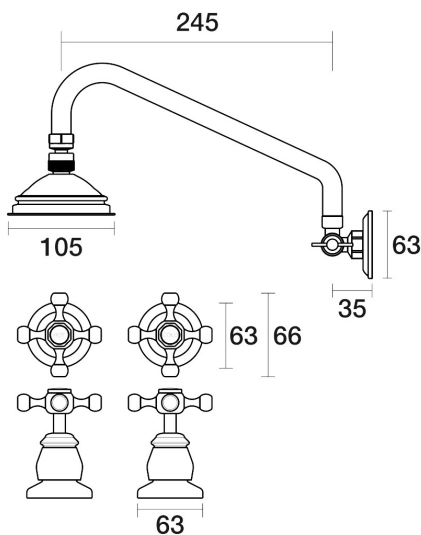
Tudor Shower Set Adjustable Arm Ceramic Disc B31.031.2.34 - Matt Black
