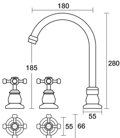
Tudor Sink Set Hob Swivel B31.051.1.03 - Chrome / White
