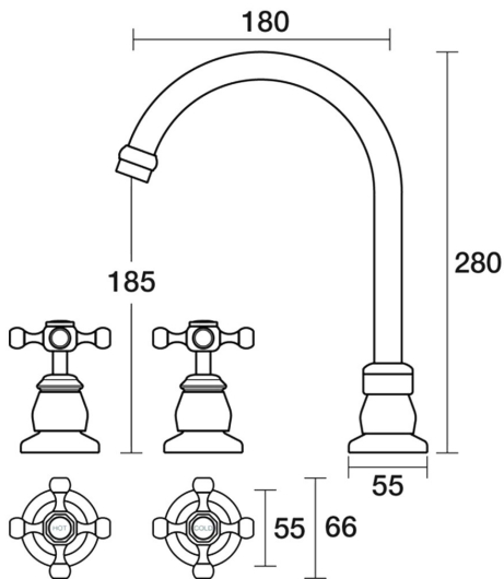
Tudor Sink Set Hob Swivel B31.051.1.26 - Black Sapphire
