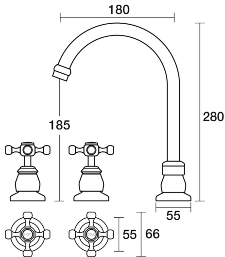
Tudor Sink Set Hob Swivel Ceramic Disc B31.051.2.57 - Matt Nickel
