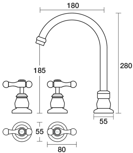
Tudor Sink Set Hob Swivel Lever Ceramic Disc B31.051.3.32 - Midnight Black
