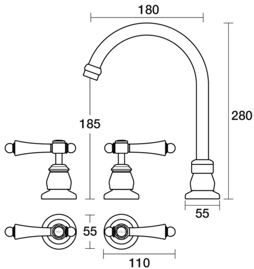
Tudor Sink Set Hob Swivel Porcelain Lever Ceramic Disc B31.051.4.12 - 23k Brushed Gold
