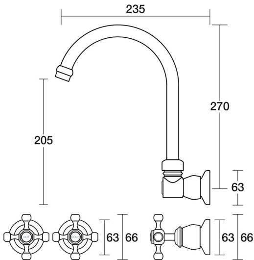
Tudor Sink Set Wall Swivel B31.052.1.24 - Brushed Gunmetal
