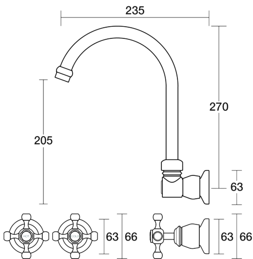
Tudor Sink Set Wall Swivel Ceramic Disc B31.052.2.01 - Chrome
