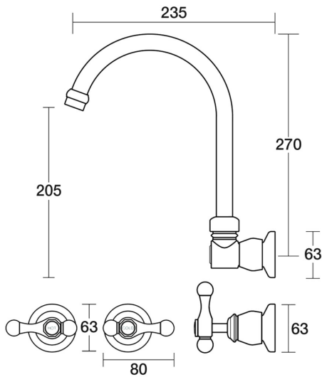
Tudor Sink Set Wall Swivel Lever Ceramic Disc B31.052.3.13 - Gold / White
