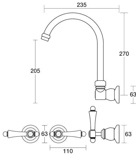
Tudor Sink Set Wall Swivel Porcelain Lever Ceramic Disc B31.052.4.01 - Chrome
