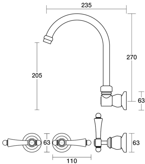
Tudor Sink Set Wall Swivel Porcelain Lever Ceramic Disc B31.052.4.40 - Rumbled Brass
