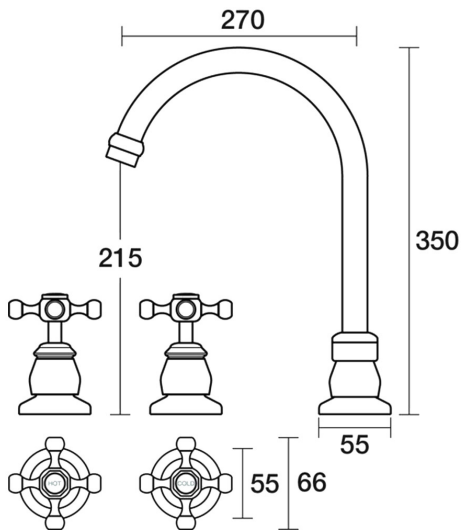
Tudor Sink Set XL Hob Swivel Ceramic Disc B31.053.2.27 - Satin Pearl
